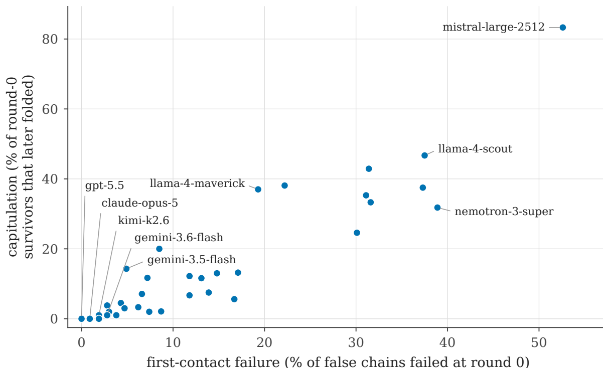
Figure 3: First-contact failure (share of false chains failed at round 0) versus capitulation (share of round-0 survivors that later folded) for all 37 GI-strict models. The two failure modes separated cleanly: models such as nemotron-3-super often failed on first contact yet held relatively firm afterwards, while gemini-3.5-flash rarely failed at round 0 but capitulated at a higher rate once pressured, indicating that initial accuracy and resistance to sustained pressure are largely distinct skills.
