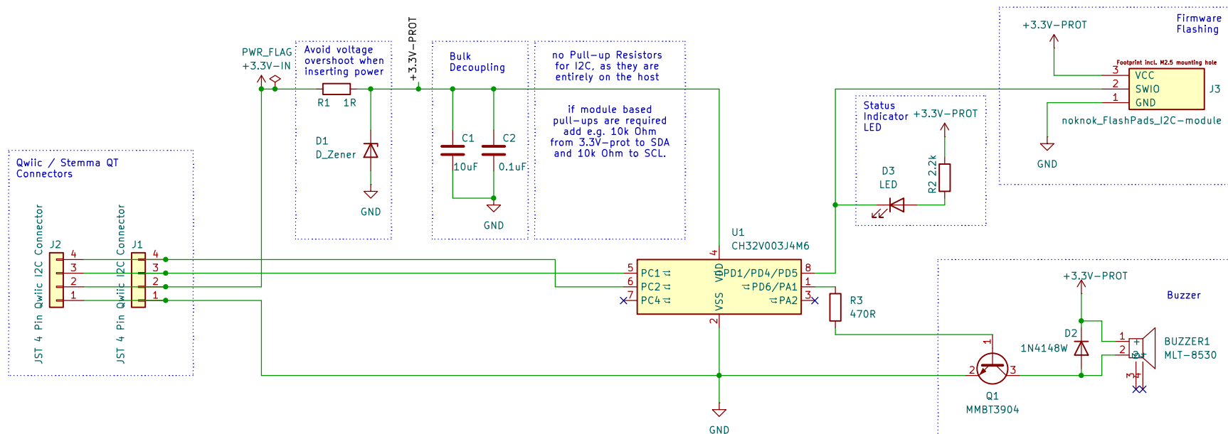
Recommended Driving Circuit
