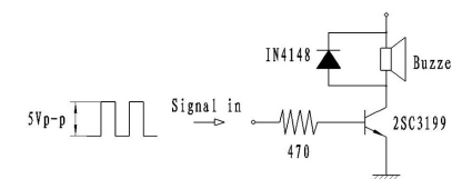
Recommended Driving Circuit
