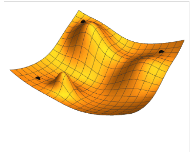
Illustration of gradient descent for three different starting points; two parameters (represented by the plan coordinates) are adjusted in order to minimize the loss function (the height). [77]
