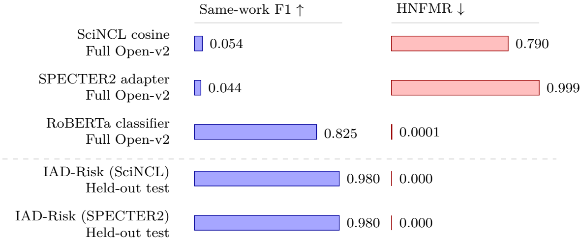
Figure 2: Open-v2 mechanism-evidence profile. The bars visualize Table 6 without changing its interpretation boundary: full Open-v2 rows and held-out test rows remain scope-labeled, and the figure supports the false-merge-control reading rather than a same-scope comparative ranking.
