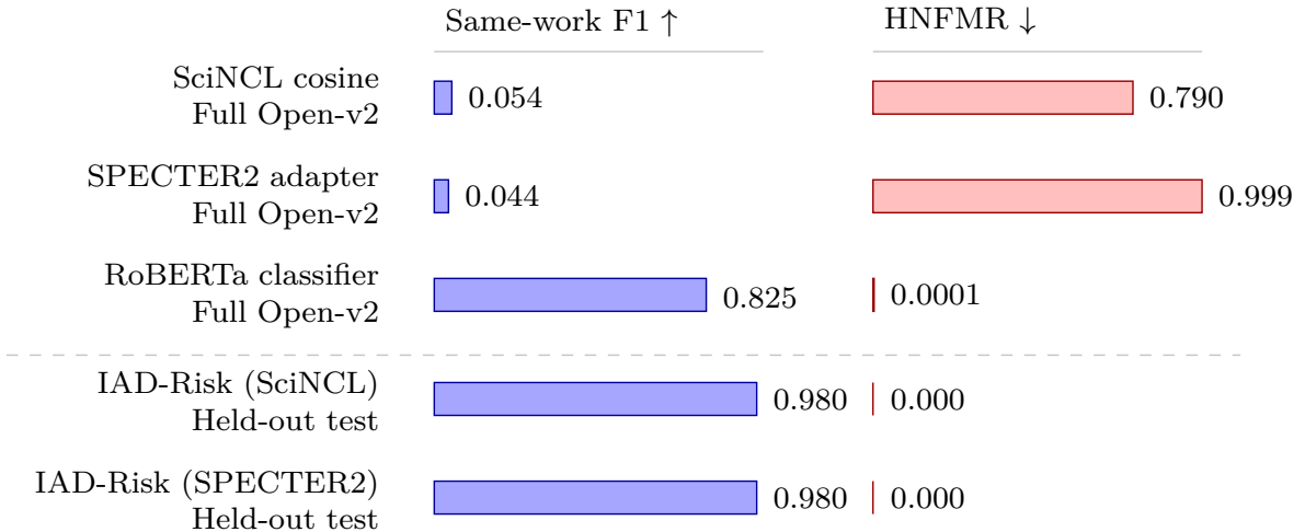
Figure 2: Open-v2 mechanism-evidence profile. The bars visualize Table 16 without changing its interpretation boundary: full Open-v2 rows and held-out test rows remain scope-labeled, and the figure supports the false-merge-control reading rather than a same-scope comparative ranking.
