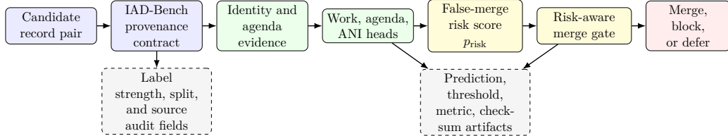
Figure 1: IAD-Risk pipeline. The framework first anchors each candidate pair in the IAD-Bench provenance contract, separates identity evidence from agenda evidence, predicts work, agenda, and ANI heads, derives a false-merge risk score, and then applies a conservative merge gate. Dashed audit nodes mark the schema fields and external artifacts required to reproduce prediction, threshold, metric, and checksum evidence.
