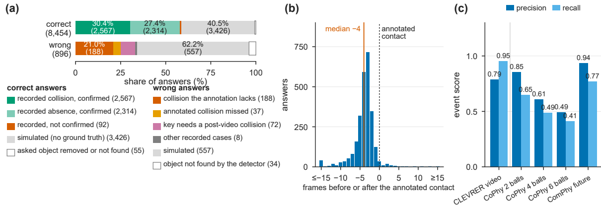
Figure 5: The evidence behind each answer. (a) Most correct answers rest on an event that can be checked against CLEVRER’s annotation, and 98.2% of those checks pass; the rest are decided in simulation, where no ground truth exists. (b) The deciding collision is found a median of 4 frames before the annotated contact. (c) Reported events against true events: recorded CLEVRER videos, simulated CoPhy counterfactuals with 2 to 6 balls, and simulated ComPhy futures.
