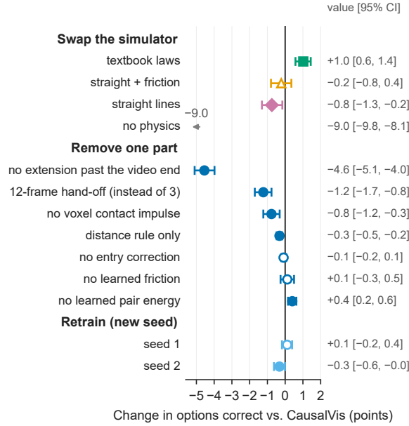
Figure 4: Effect of each change on the full system. Points are paired differences in options correct on TEST-A and TEST-B with 95% video-bootstrap intervals; filled markers exclude zero. The extension past the video end and the hand-off timing matter most; the learned parts matter little, and removing the learned pair energy helps.
