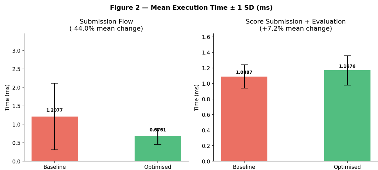
Figure 4: Figure 2 Mean Execution Time \pm 1 SD
