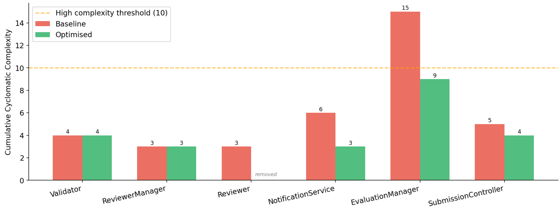
Figure 6 — Cumulative Cyclomatic Complexity per Class
