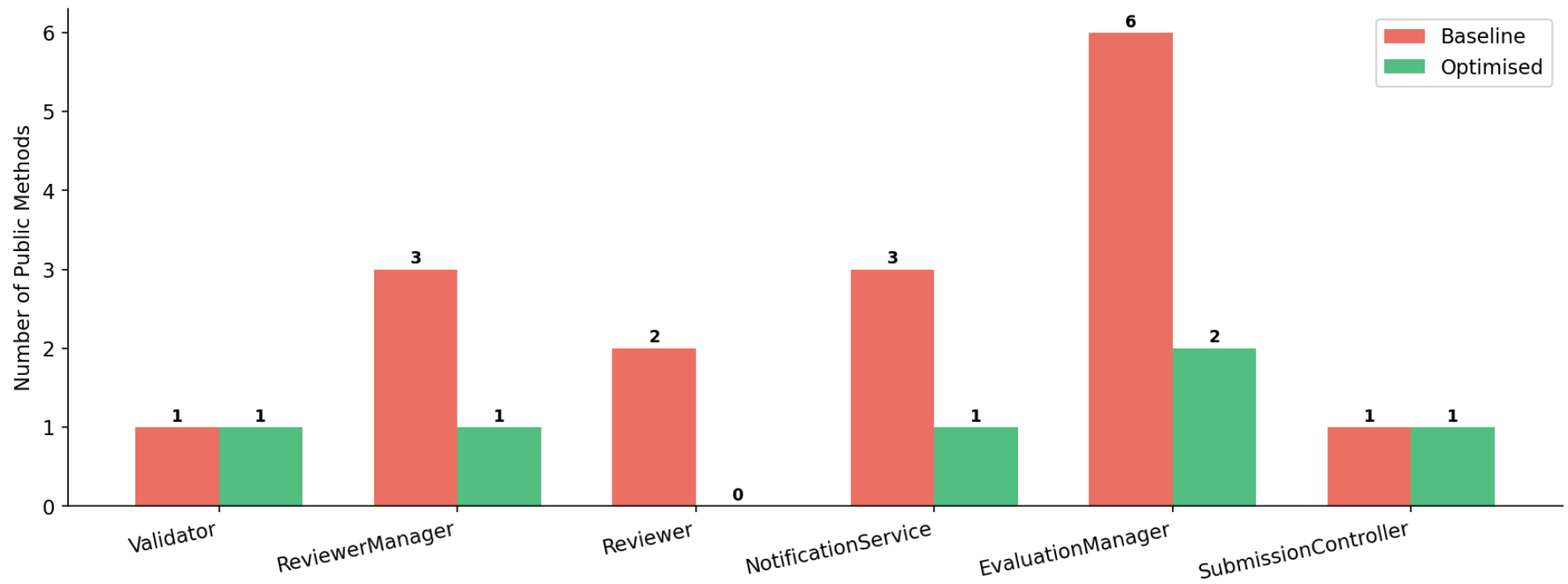
Figure 7 — Public Methods per Class
