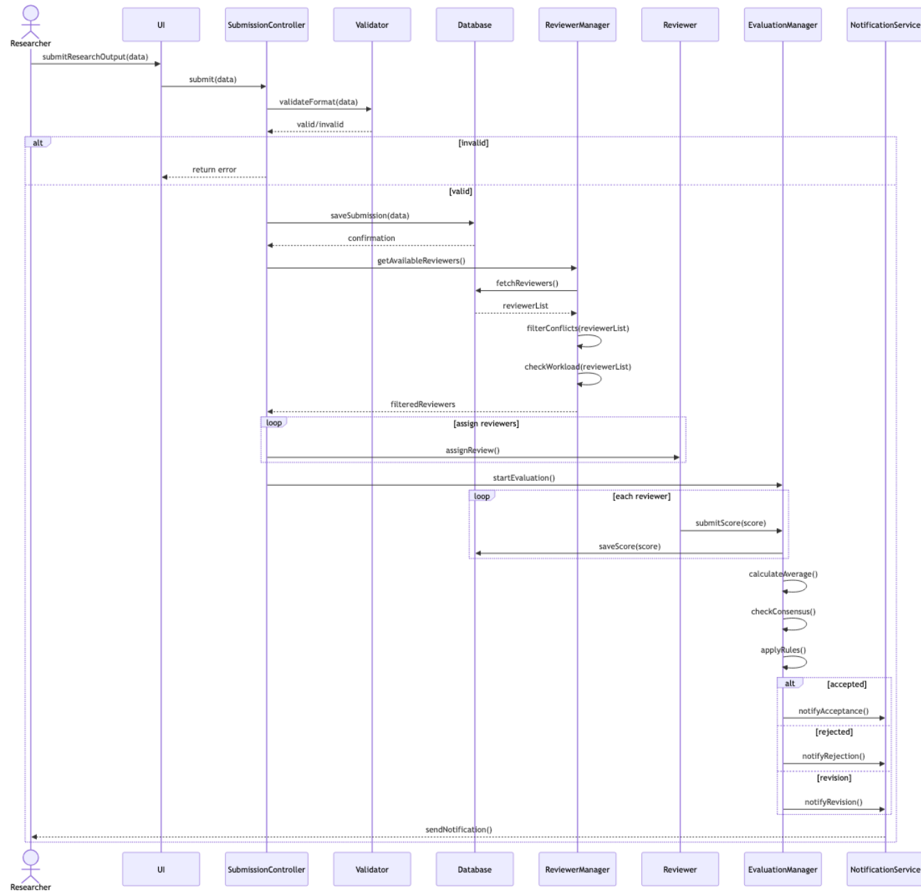
Figure 1: Baseline Sequence Diagram
