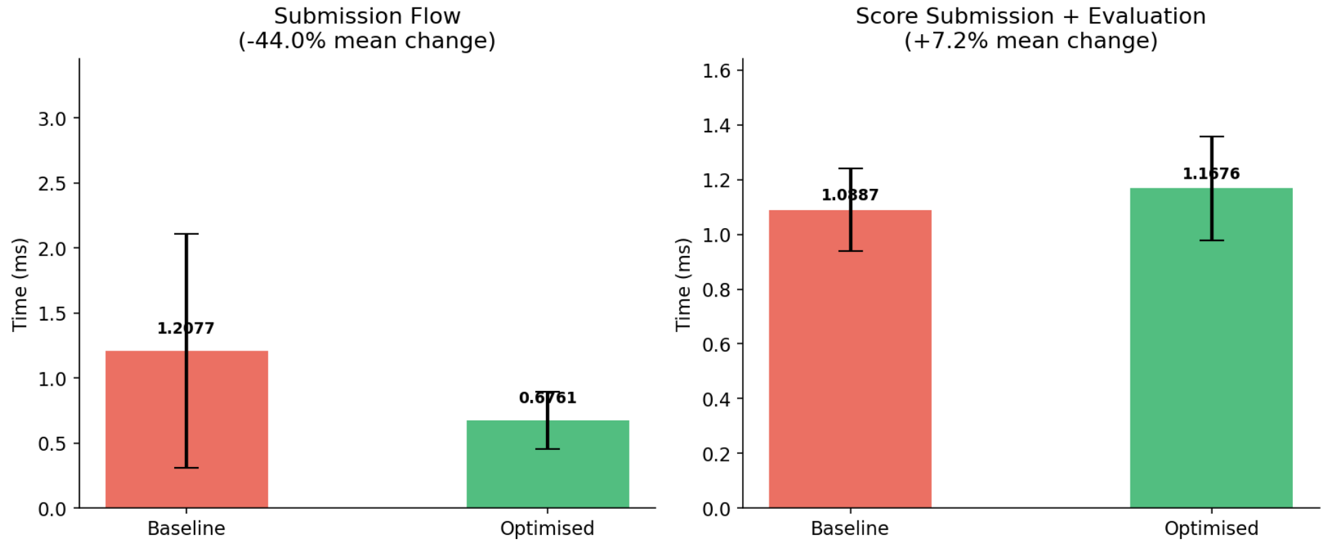
Figure 6: Figure 2 Mean Execution Time \pm 1 SD
