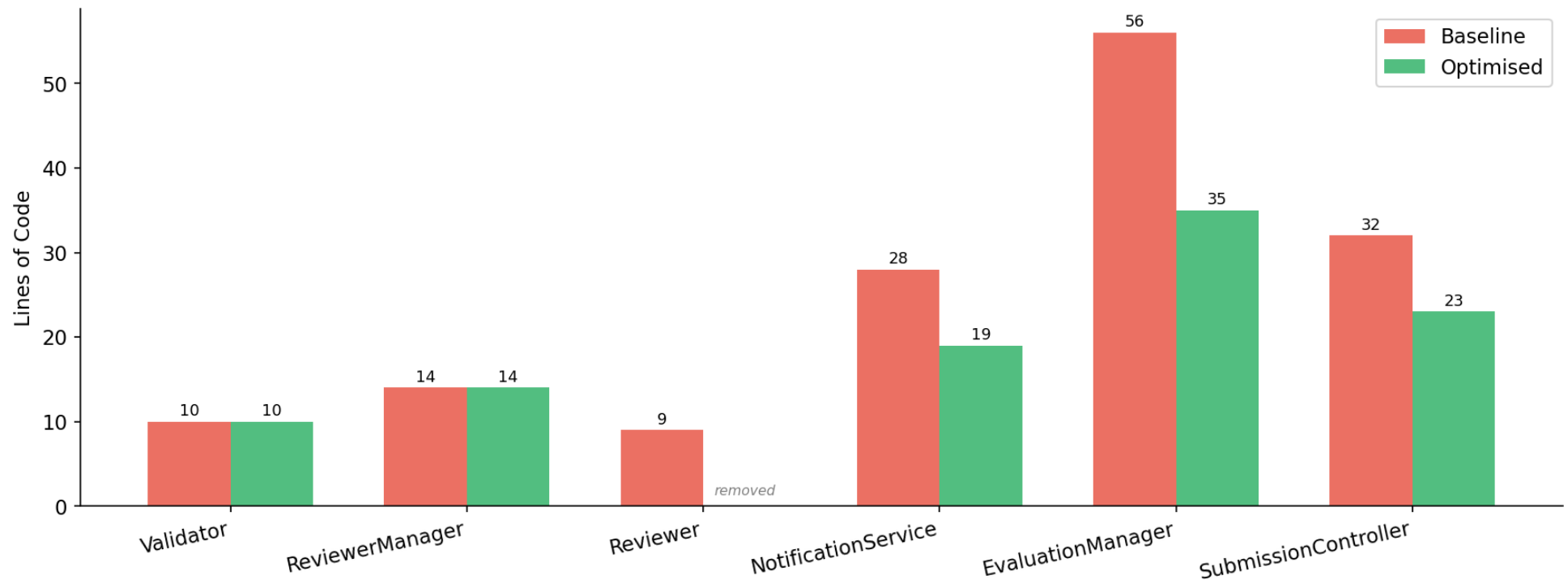
Figure 5 — Lines of Code per Class (controllers.py)
