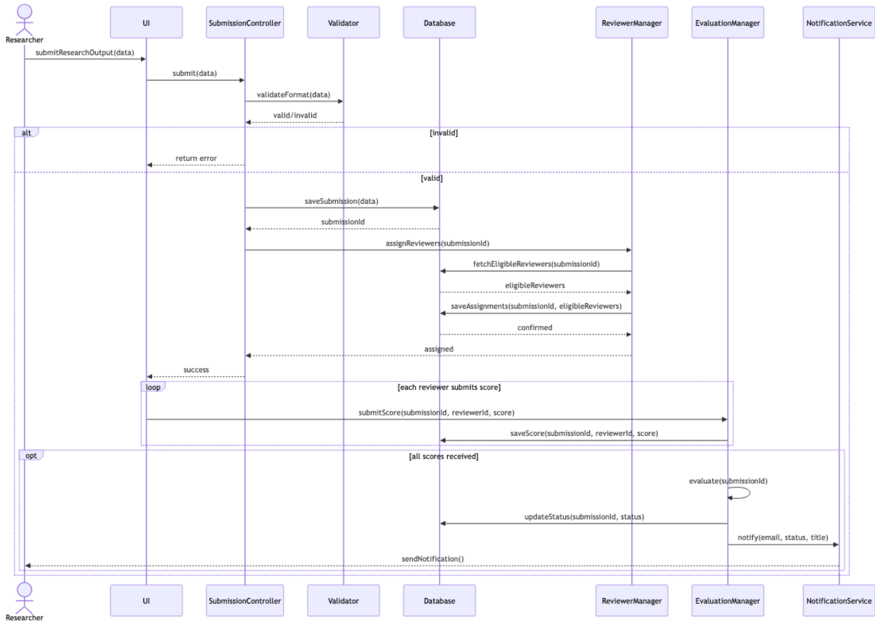
Figure 3: Optimised Sequence Diagram
