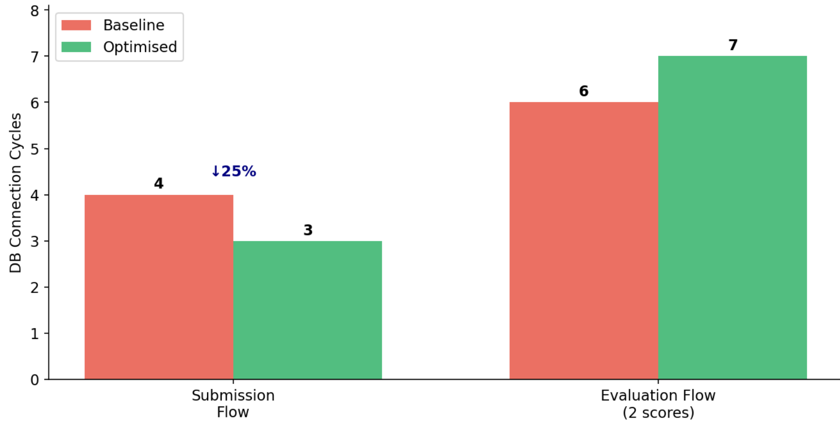
Figure 6: Figure 4 Database Connection Cycles per Operation
