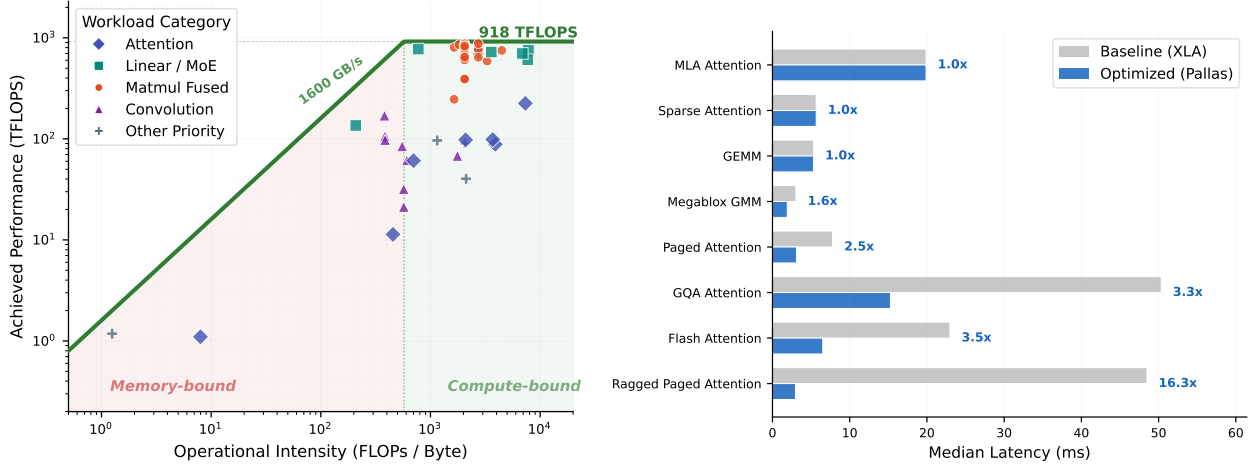
(a) TPU v6e roofline [30] with all 50 workloads. (b) Tokamax Pallas kernel speedup over XLA.
