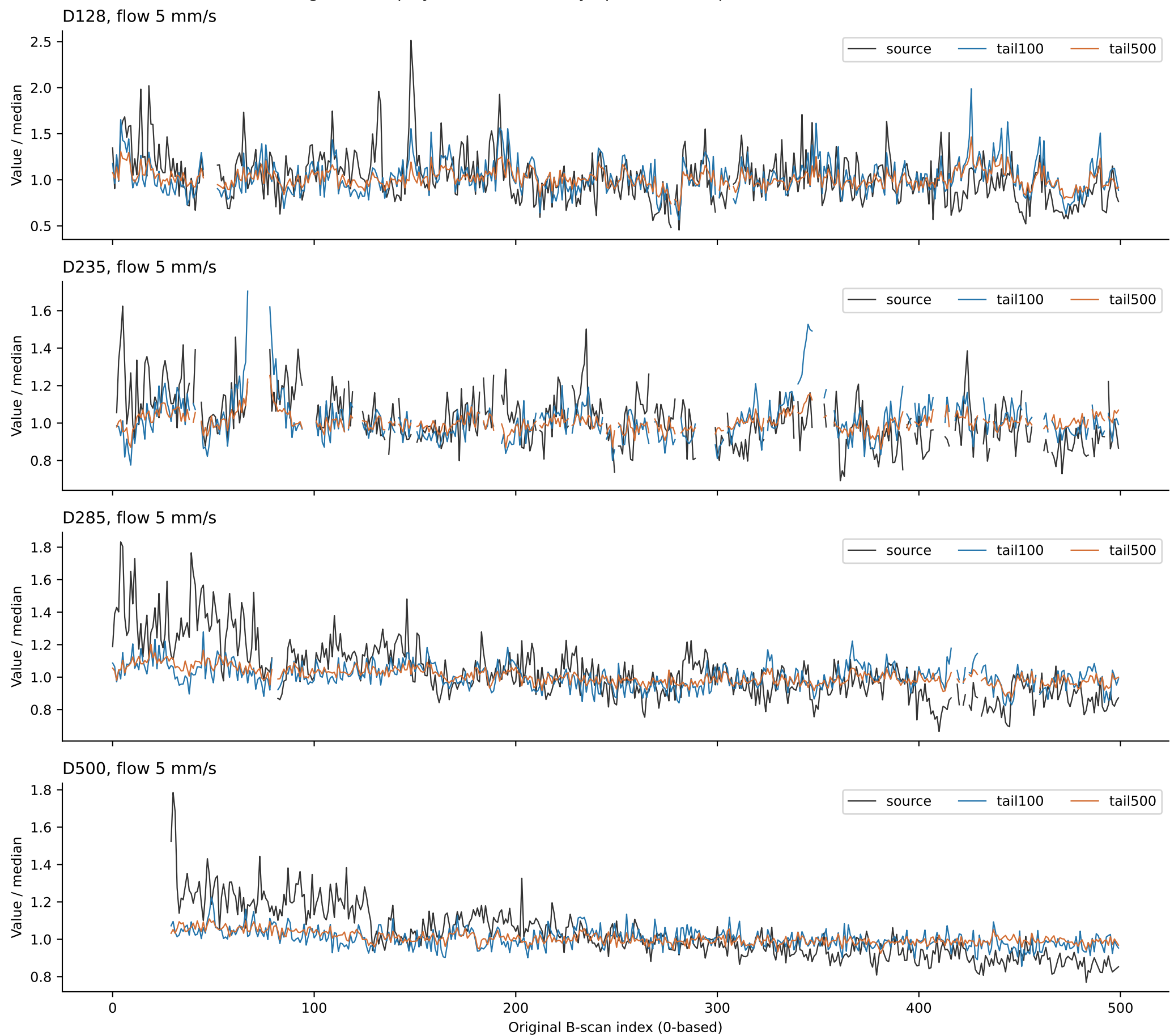
Figure 1. Display normalization only; quantitative input is linear raw SV
