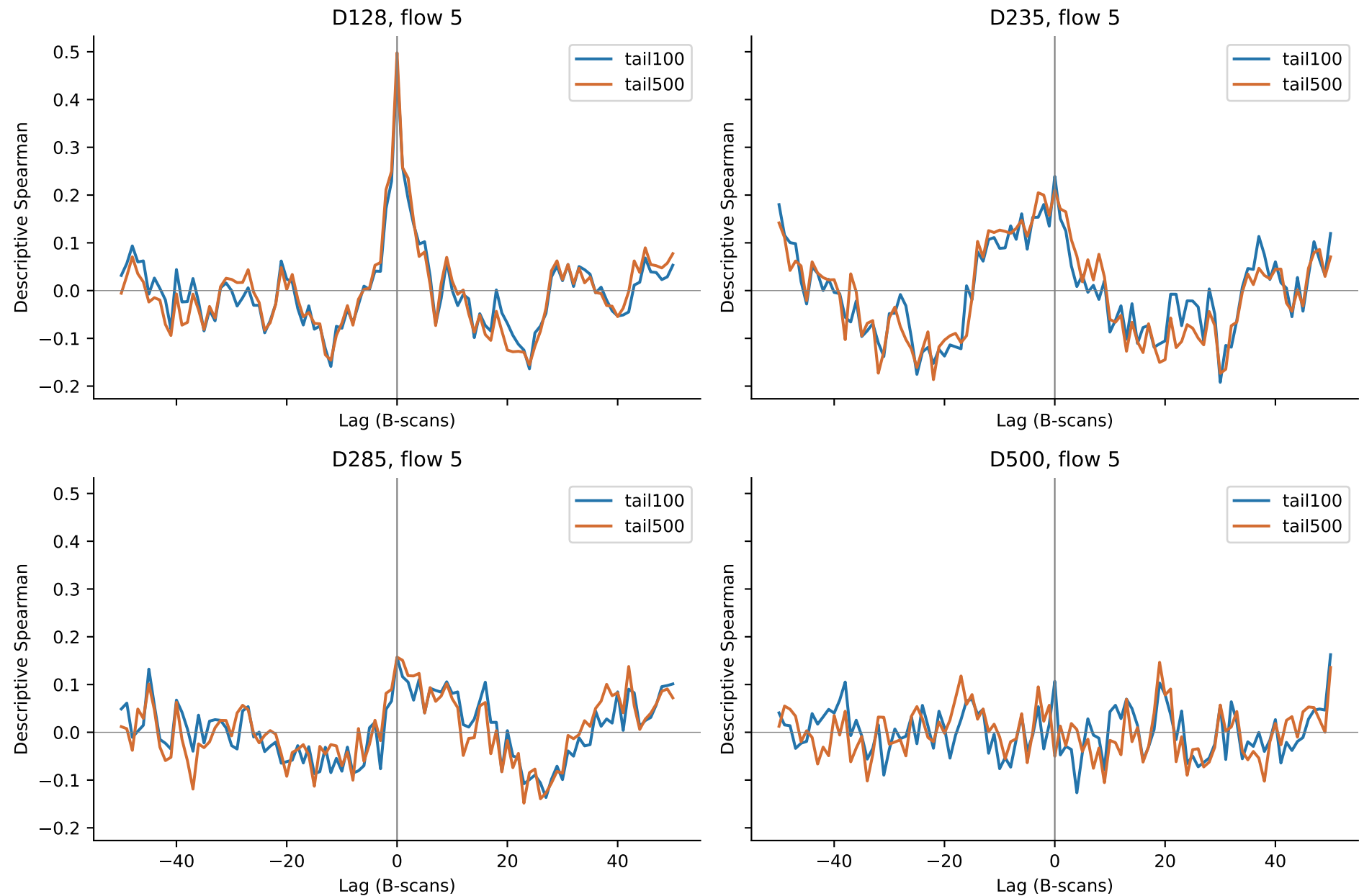
Figure 3. Source mean / tail mean: detrended_51
