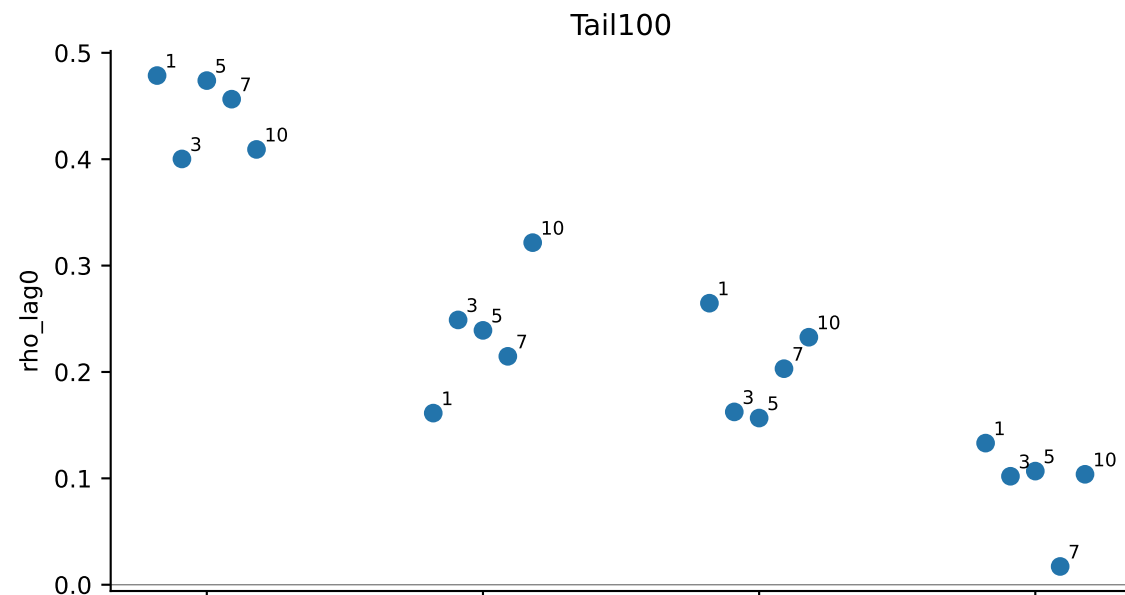
Figure 4. 51-frame residuals; every common-flow volume (labels = mm/s)
