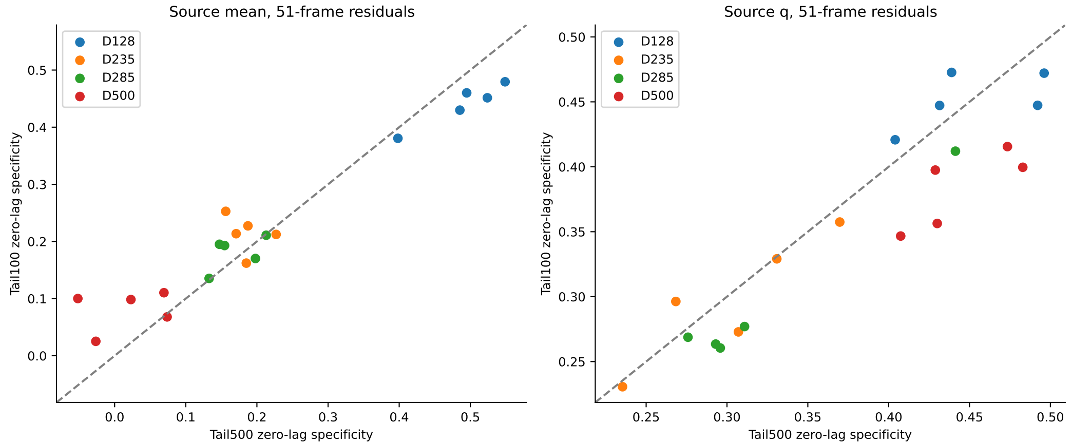
Figure 6. Matched tail-depth comparison; all 20 common-flow volumes
