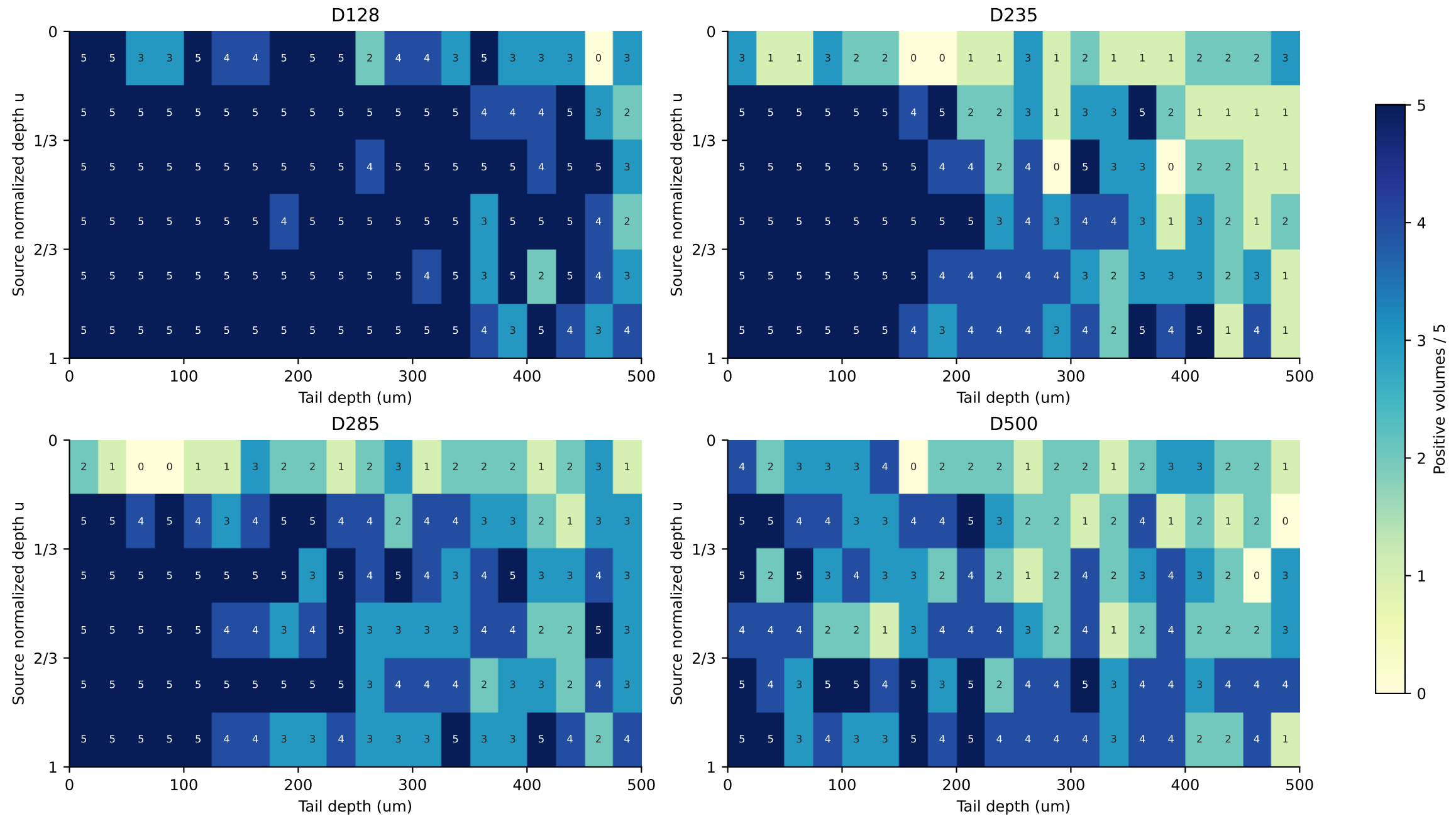
Figure 2. Number positive out of five common flows
