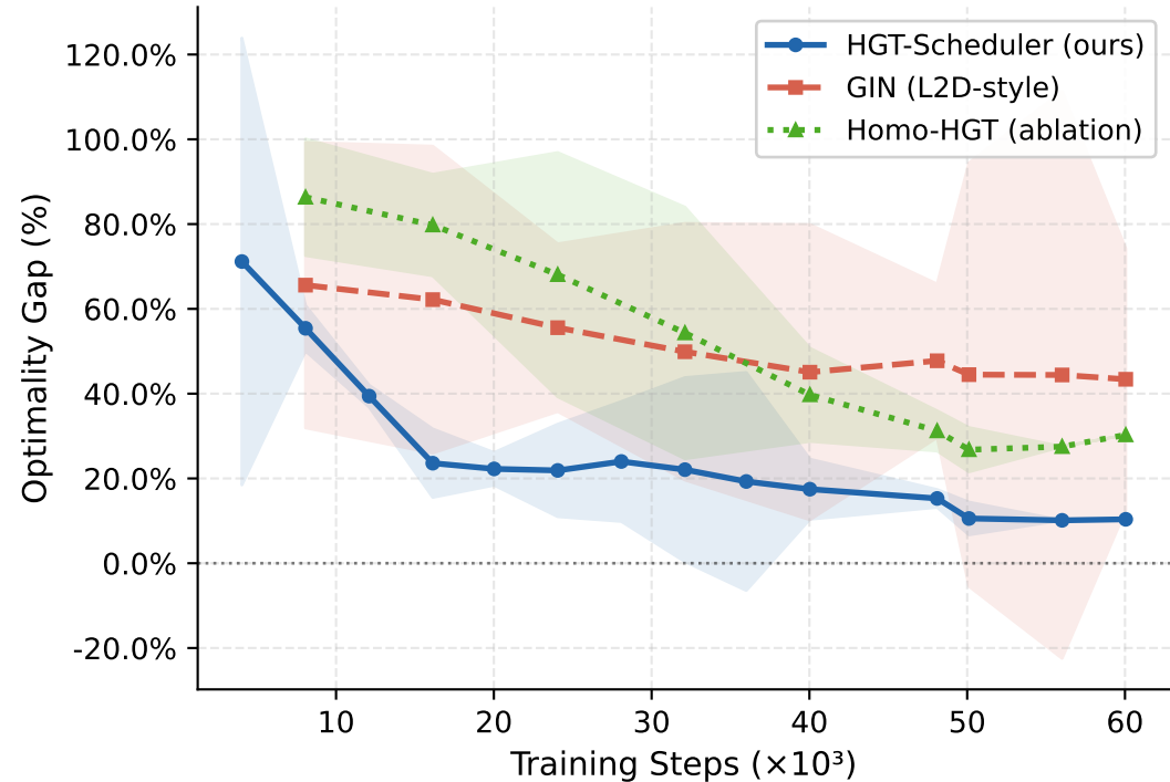
FT06 (6×6)
