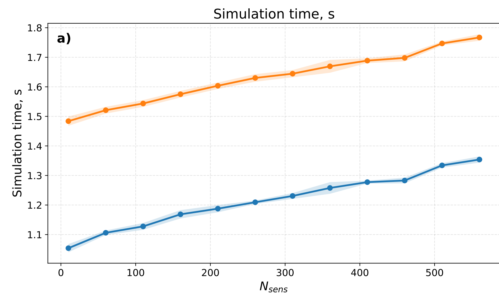
lorenz: PC-SC vs PC-EC mean \pm std over 10 tests
