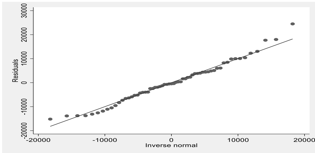
Fig. 14: Q-Q Plot of Residuals from the ARDL Model of Coffee Exports
