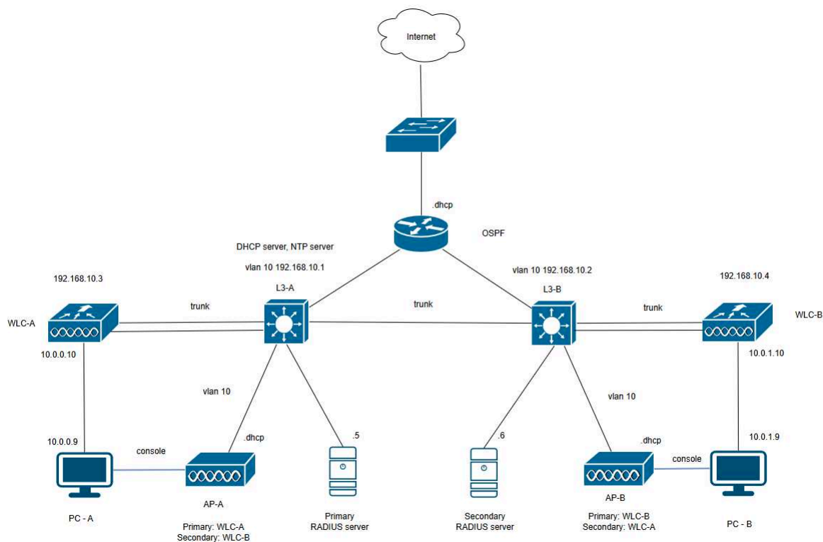
Figure 12: Lab three exercise topology
