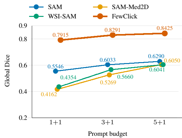
Figure 4: Global Dice versus prompt budget on the common 885 occurrences (819 unique patches). Methods share targets, masks, negative points, and prefixes of the same frozen positive-point sequence.
