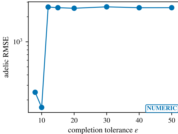
Adelic completion vs \varepsilon
