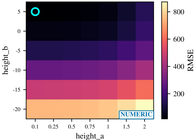
Adelic RMSE height map
