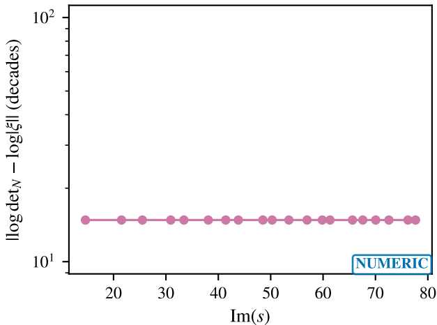
Spectral determinant vs completed \xi along the strip
