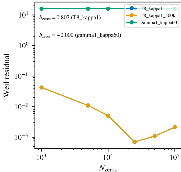
Weil explicit formula convergence
