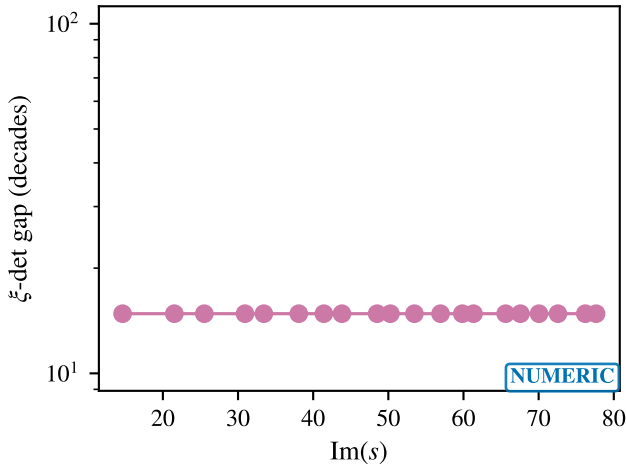
Spectral determinant vs completed \xi
