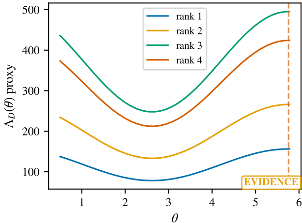
Spectral action by rank
