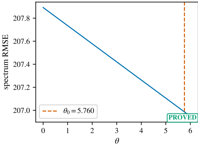
Spectral action \Lambda_D(\theta) proxy
