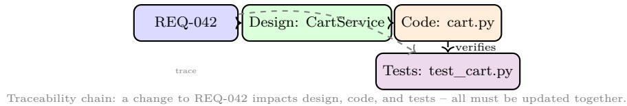
Figure 7.3: Impact analysis via traceability – a requirement change propagates through design, code, and tests; missing any link is a defect.
