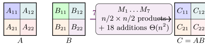
Figure 4.2: Strassen: one n \times n product reduced to seven n/2 \times n/2 products plus O(n^2) additions.
