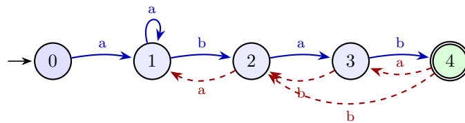
Figure 7.2: KMP automaton for P = \text{abab} ( m = 4 ). Solid spine spells P ; failure links (merged into \delta ) redirect on mismatch via \pi : \pi = [0, 0, 1, 2] . Scanning T never moves backwards, giving O(n + m) time.
