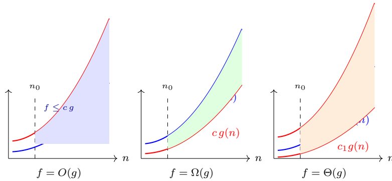
Figure 2.1: O , \Omega , and \Theta as eventually-sandwiching bands. Only behaviour for n \geq n_0 matters; constants c, c_1, c_2 scale the reference g(n) .
