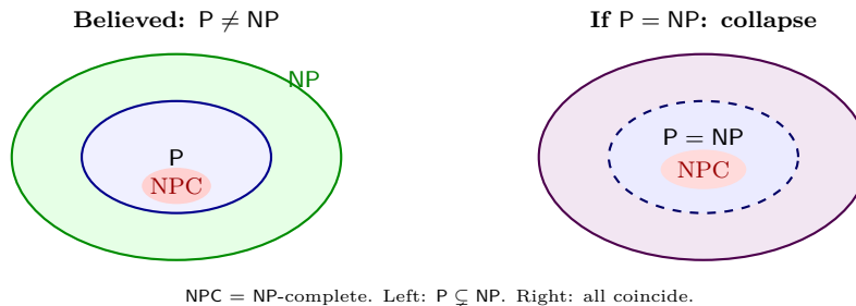
Figure 8.6: Two views of P vs. NP . Left is widely believed; right would make every NP problem tractable.
