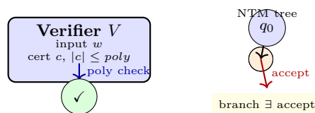
Figure 8.2: Two views of NP : poly-time verifier with short certificate vs. poly-time NTM with existential branching; they are equivalent via “certificate = nondeterministic choices”.
