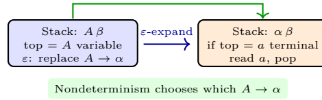
Figure 5.3: CFG \rightarrow PDA: expand variables via \varepsilon -moves; match terminals against input. Every leftmost derivation corresponds to a PDA computation and vice versa.
