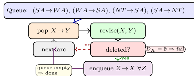
Figure 4.3: AC-3 queue processing. Each revise may shrink D_X ; neighbours are re-enqueued only on deletion. Coloured stages show queue \rightarrow revise \rightarrow enqueue cycle until fixpoint.
