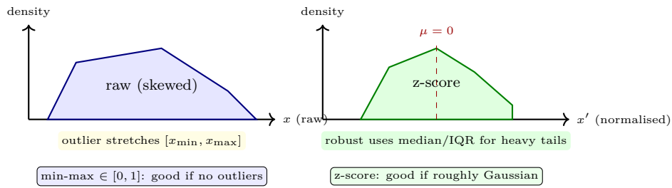
Figure 2.2: Normalisation choices. Min-max preserves distribution shape but an outlier compresses all other points; z-score centres at zero; robust scaling survives outliers.
