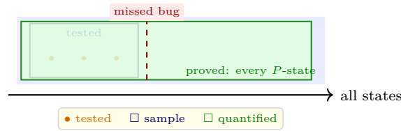
Figure 1.2: Testing samples finitely many points (orange dots) inside the blue sample box; proof shades the entire green region. A bug lurking outside the sample is invisible to tests but caught by proof.
