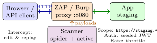
Figure 7.2: Proxy-based DAST. The proxy sees plaintext HTTP, can spider the app, inject payloads, and replay with modified auth/params.
