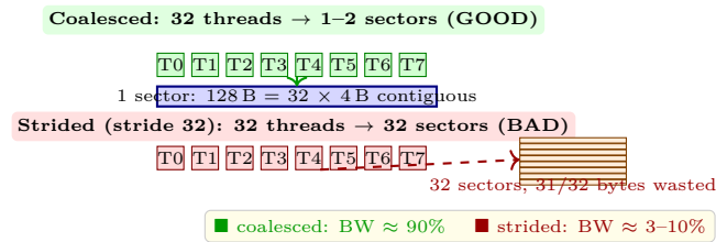
Figure 3.2: Coalescing: contiguous warp accesses collapse to one transaction; strided/random accesses explode to many. Structure-of-arrays and transposed layouts exist to restore coalescing.
