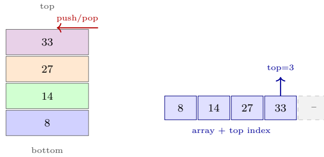
Figure 2.1: Stack plates (LIFO) and array implementation with top pointer. Linked-list version uses head as top.
