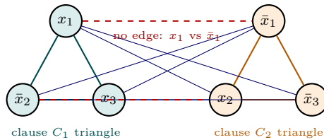
Figure 8.3: 3SAT \rightarrow CLIQUE gadget: one triangle per clause; connect compatible literals across clauses (omit conflict edges x-\bar{x} ). An m -clique picks one literal per clause with no conflicts iff \phi is satisfiable.
