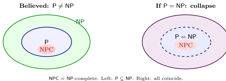
Figure 8.6: Two views of \text{P} vs. \text{NP} . Left is widely believed; right would make every \text{NP} problem tractable.
