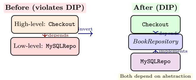
Figure 5.3: DIP: introduce an abstraction so high-level policy does not depend on low-level detail; both depend on the interface.
