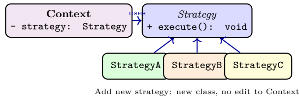
Figure 6.1: Strategy pattern: Context delegates to a Strategy interface; new behaviours are new classes (OCP).
