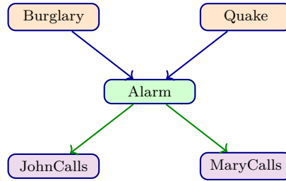
Figure 6.4: Alarm network: burglary and earthquake cause the alarm; calls depend only on it. Five small tables replace a 32-entry joint.
