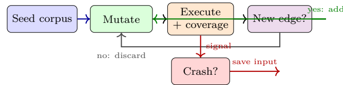
Figure 5.1: Coverage-guided fuzzing loop. Coverage feedback retains only inputs that expand the frontier; sanitizers turn silent corruption into a crash so the fuzzer notices it.
