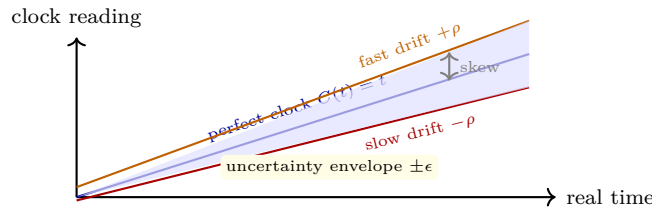
Figure 2.1: Physical clocks diverge within a drift envelope. NTP/PTP/TrueTime bound the skew but never eliminate it.
