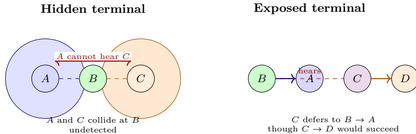
Figure 7.1: Left: hidden terminal — A and C hidden from each other collide at B . Right: exposed terminal — C is needlessly blocked. Both motivate RTS/CTS and carrier sensing.
