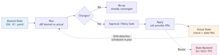
Figure 4-1: The declarative convergence loop — desired state in Git is diffed against actual state (cloud + state file); the plan is gated and applied; drift detection re-enters the loop on a schedule.
