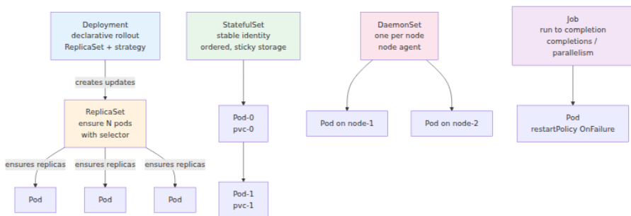
Figure 3-2: Workload controller taxonomy — Deployments manage ReplicaSets for stateless rollouts; StatefulSets provide ordered identity; DaemonSets run per-node agents; Jobs run to completion.
