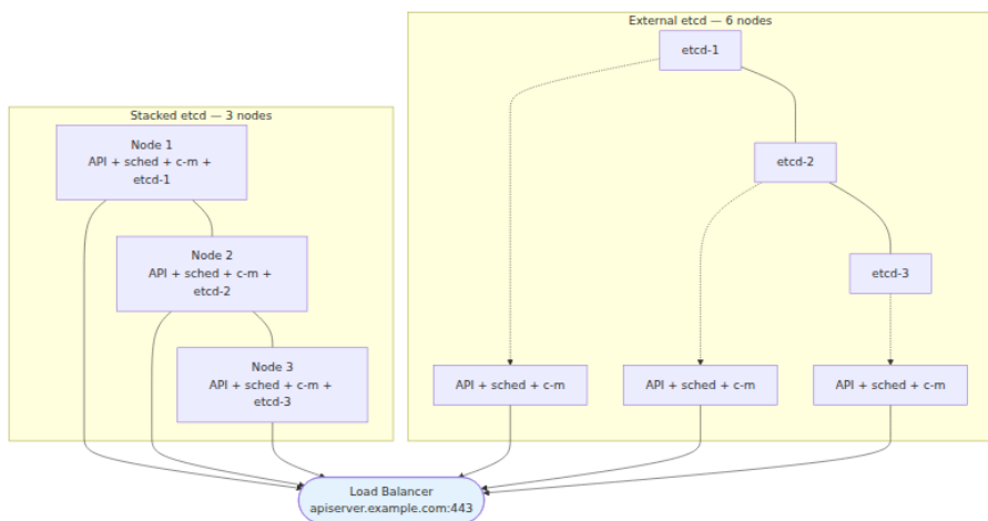
Figure 2-2: Stacked vs. external etcd — stacked is simpler but couples etcd to control-plane load; external isolates etcd on dedicated hosts with dedicated disks.
