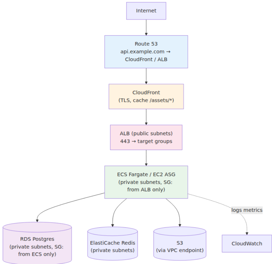
Figure 5-5: Minimal production stack on AWS — Route 53 → CloudFront → ALB → ECS/EC2 in private subnets → RDS + ElastiCache + S3, with VPC endpoints and security-group isolation.
