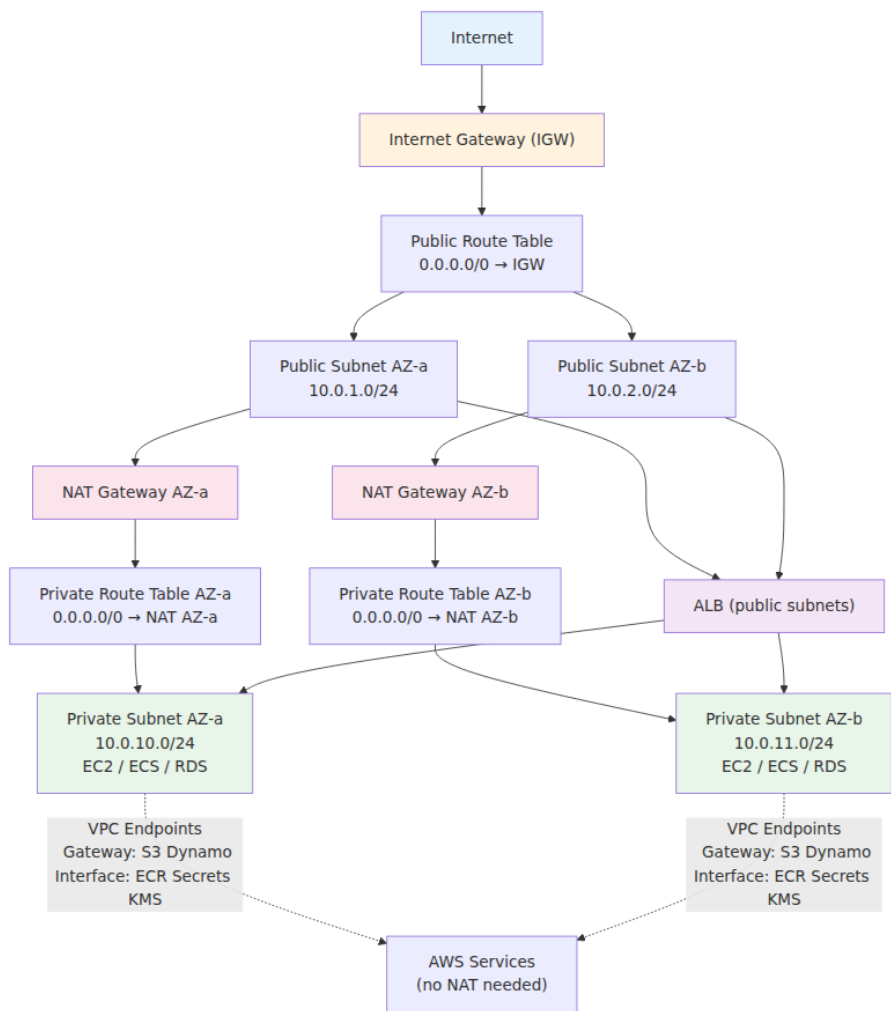
Figure 5-3: Canonical VPC layout — public subnets with IGW, private subnets with per-AZ NAT, ALB in public subnets forwarding to private workloads, and VPC endpoints for AWS services that bypass NAT.
