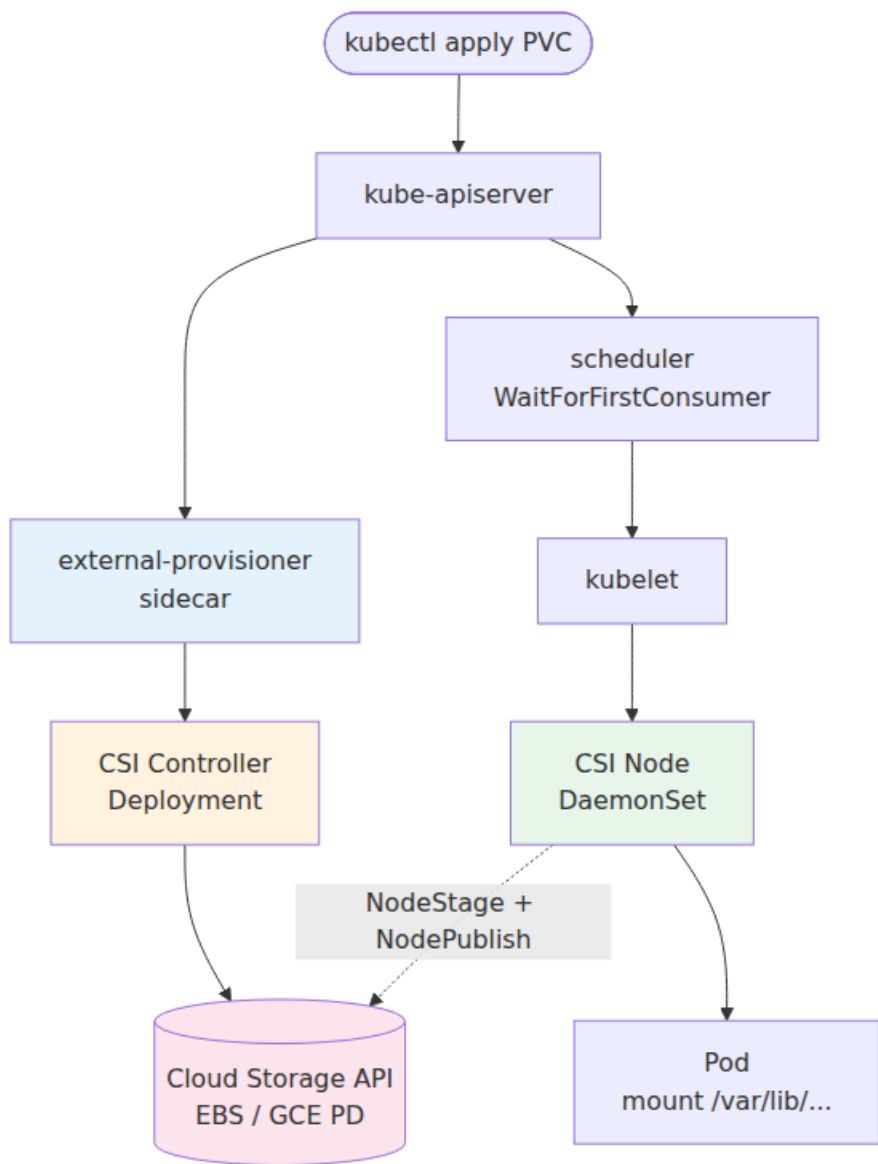
Figure 3-6: CSI volume lifecycle — external-provisioner calls the controller to create the cloud volume; after scheduling, the node driver mounts it for the pod.
