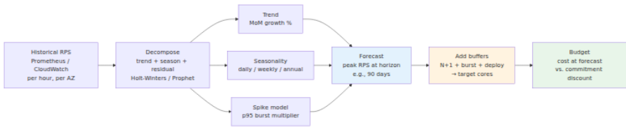
Figure 9-5: Forecasting pipeline — historical RPS is decomposed into trend, seasonality, and spike components; the forecast plus explicit buffers (N+1, burst, deploy surge) yields the capacity target and budget.
