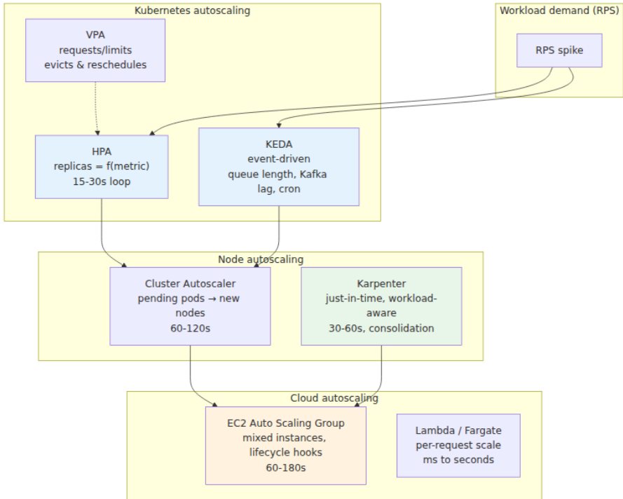
Figure 9-4: The autoscaling hierarchy — workload metrics drive pod scaling (HPA/KEDA/VPA), pending pods drive node scaling (CAS/Karpenter), and node groups are ultimately EC2 ASGs with launch templates.
