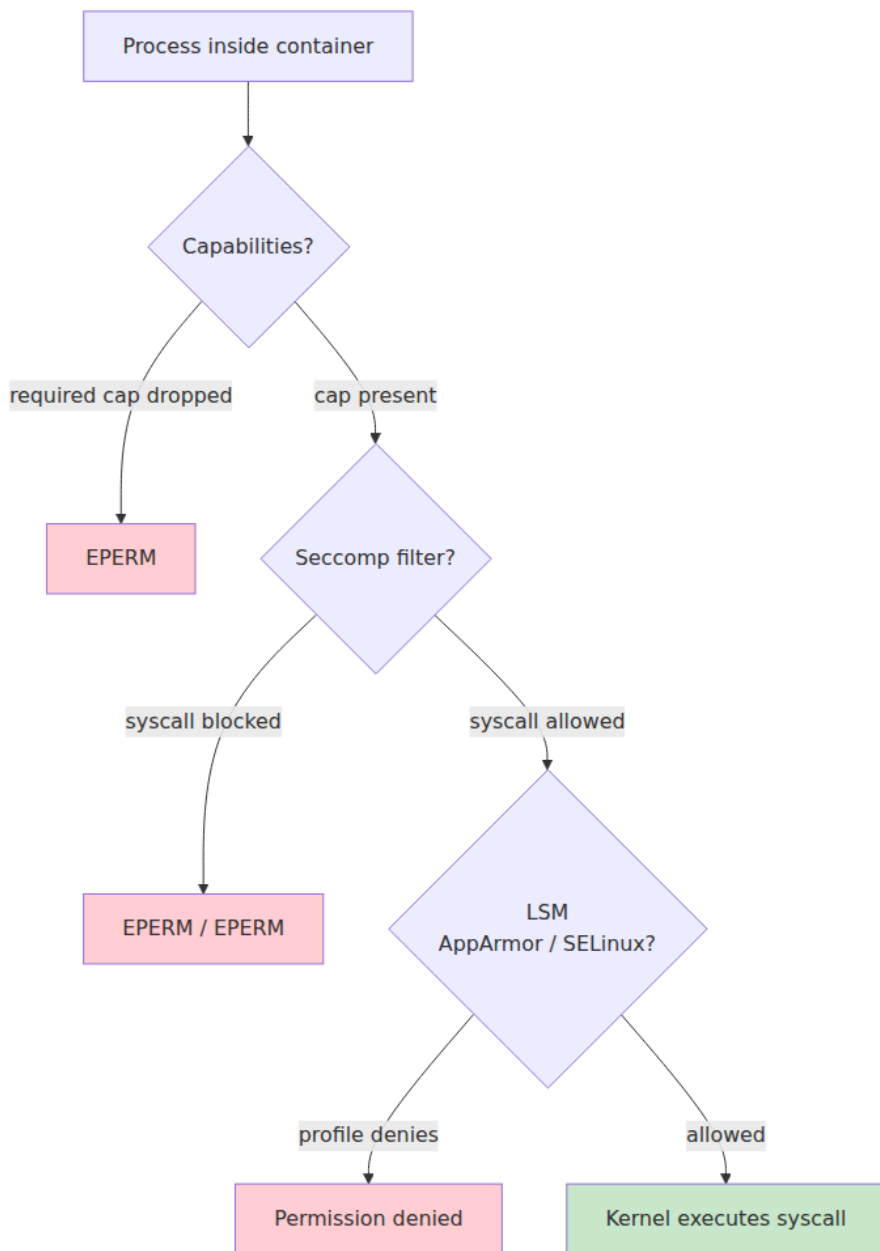
Figure 1-4: Layered syscall filtering — capabilities gate privileged operations, seccomp filters the syscall table, and LSM (AppArmor/
