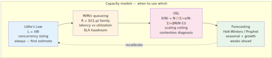
Figure 9-3: The modeling stack — Little's Law sizes concurrency, queueing sets the utilization target, USL finds the scaling ceiling, forecasting projects demand weeks out.
