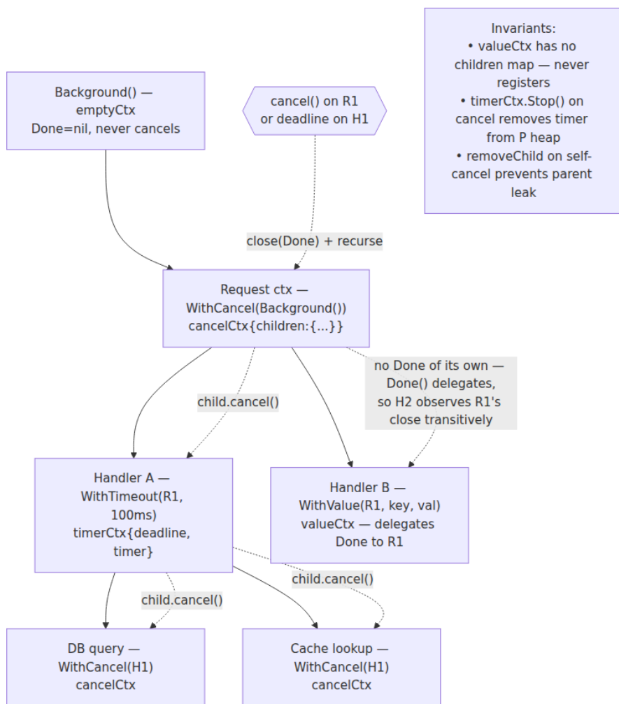
Diagram 5 — Context tree: Background root, cancelCtx/timerCtx/ valueCtx children, recursive cancel via close(Done) broadcast, delegation edges.
