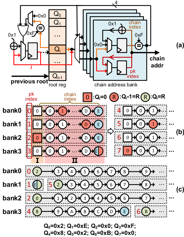
Fig. 4. (a) Unified chain address generator (b) Chain address generation in sequential mode (c) Chain address generation in out-of-order mode.
