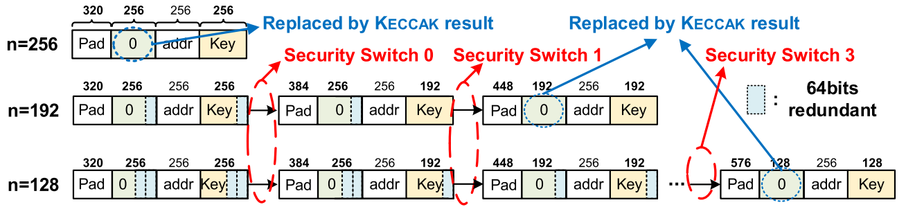
Fig. 6. Security switch process of WOTS+ in SPHINCS+ 256/192/128.
