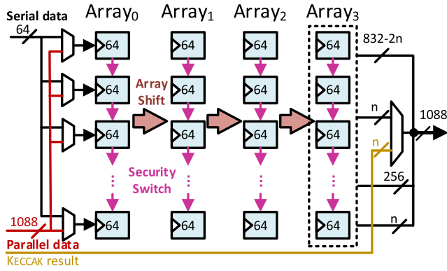
Fig. 5. Hash input logic.
