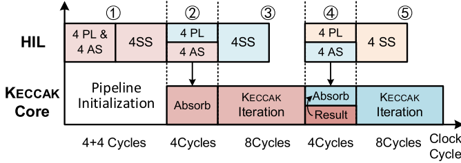
Fig. 7. Module scheduling of WOTS+ in SPHINCS+128.
