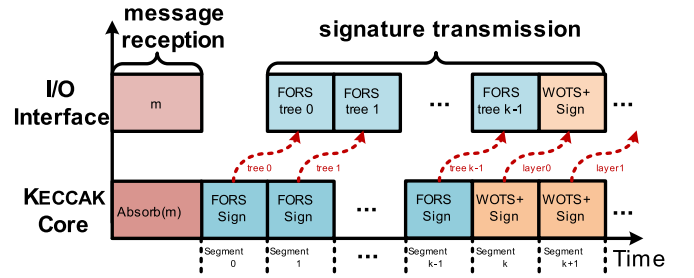
Fig. 10. Segmented signature streaming.
