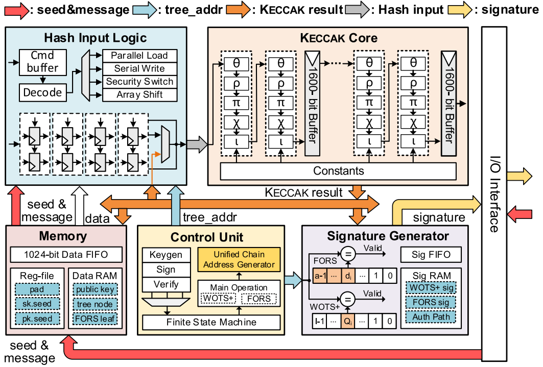
Fig. 3. Overall architecture of SPHINCS+ processor.
