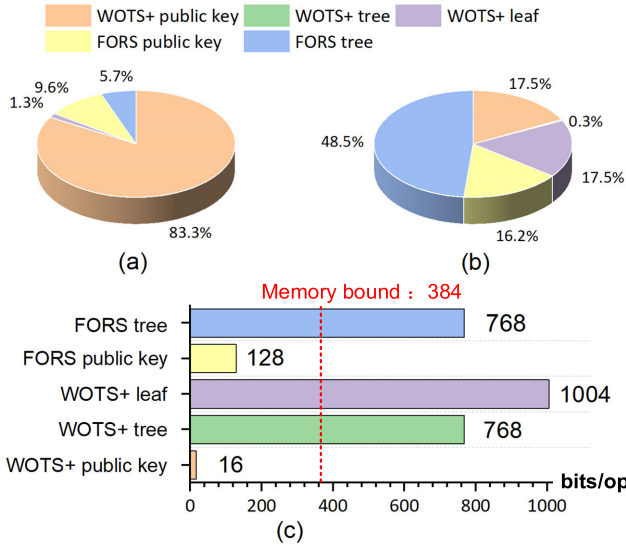
Fig. 8. Characterization of main processes. (a) Number of hash execution. (b) Number of memory access. (c) Average memory access.
