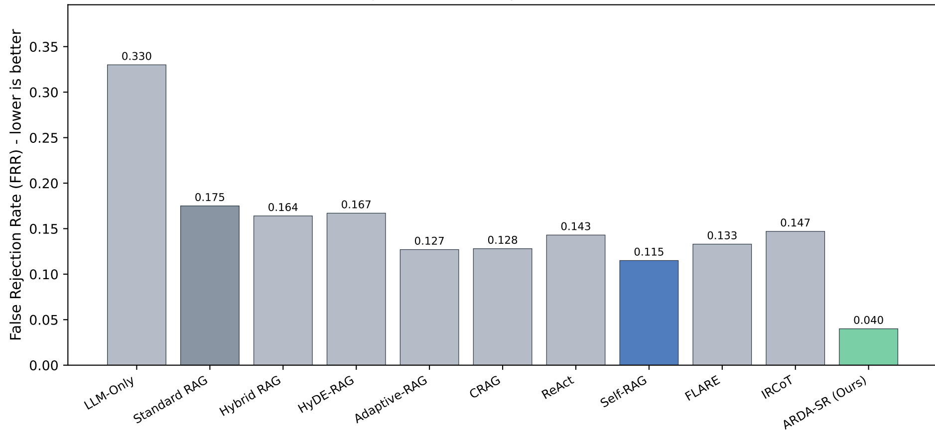
False Rejection Rate Comparison across Methods
