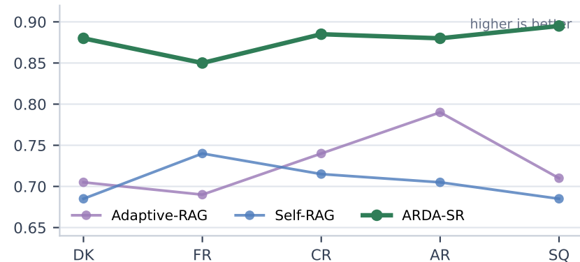
(c) Reasoning & Decision: ToolAcc
