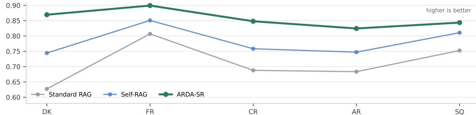
(a) Answer Quality: mean of Rel., Faith., Cov.
